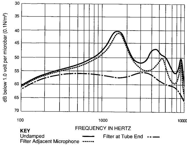
FIGURE 5. Effect of damping in 50.8mm (2") No. 13 tubing.
