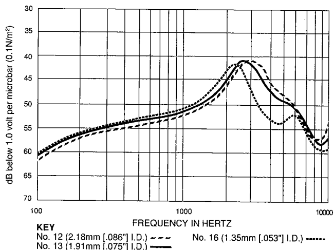
FIGURE 2. Effect of tube diameter on EK-3024 microphone. 25.4mm (1") tube length.
