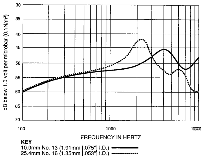
FIGURE 3. Effects of tube length and diameter combined. EK-3024 microphone.
