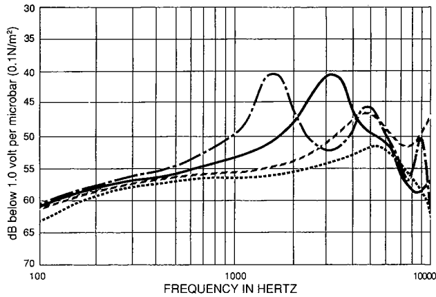
Effect of tube length on EM-3046 microphone. No. 13 Tubing.
