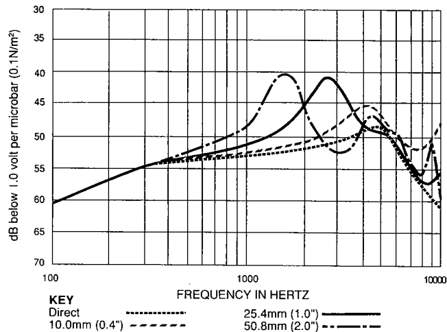
FIGURE 1. Effect of tube length on Knowles EK-3024 microphone. No.13, 1.91 mm (.075") tubing.
