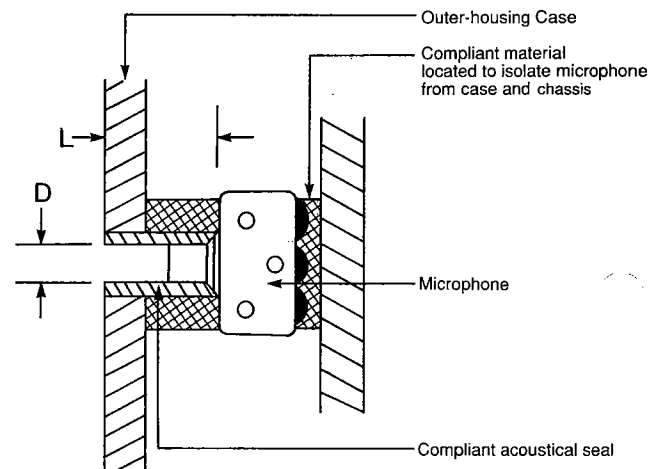
FIGURE 4. Microphone mounting cross-section.
