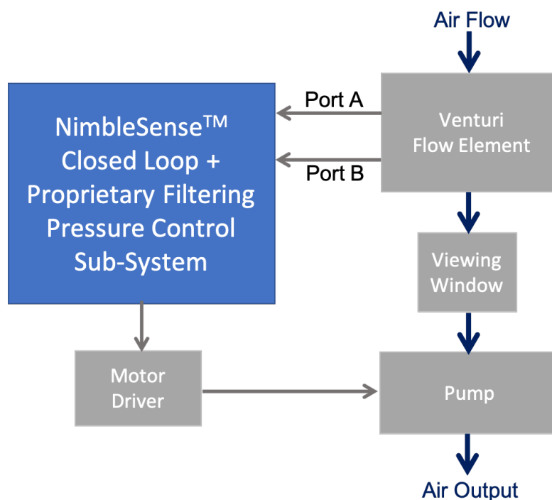
Figure 9: Closed Loop Control – Air Quality Application Example
