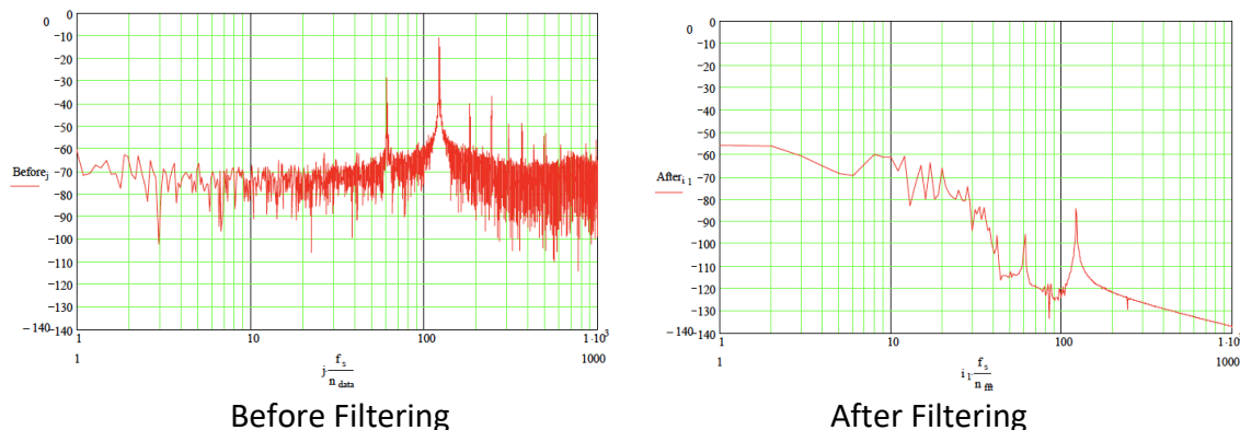
Figure 11: Before & After Results from NimbleSense 4 th Order FIR Filter
