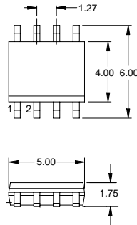
Package Configuration
