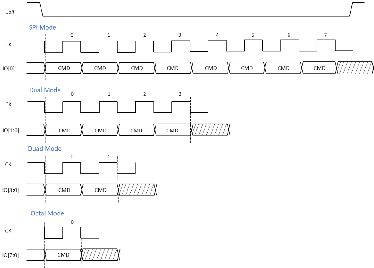
Figure 31 4-BYTE Enter/Exit
